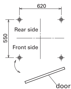
Anchor plan, door open/close diagram
