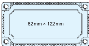
EP3 75 A (6th Generation V Series)
