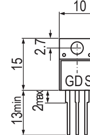
TO -220F
