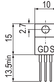
TO -220
