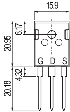
TO -247
