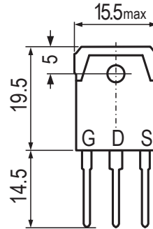
TO -3P(Q)
