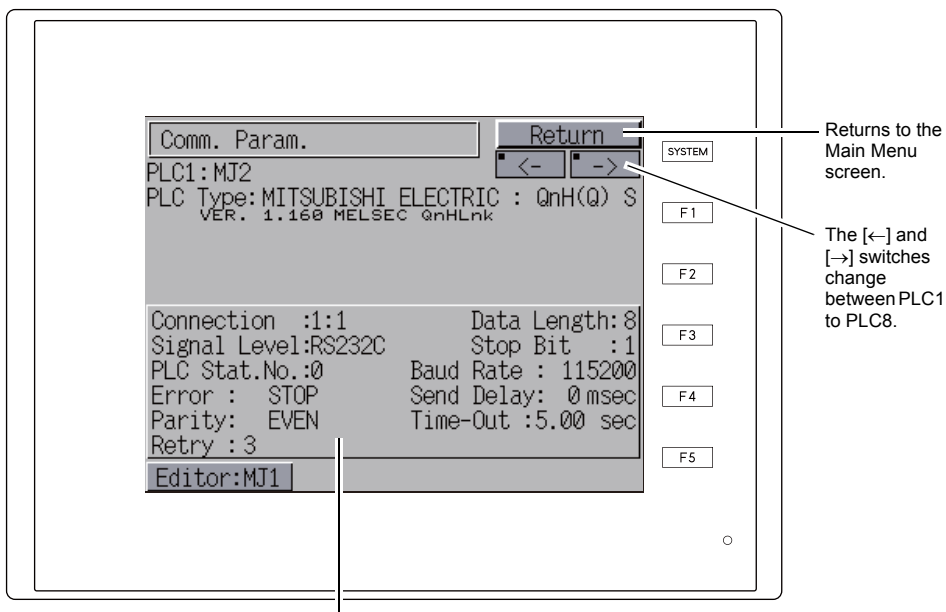
Comm. Param. screen
