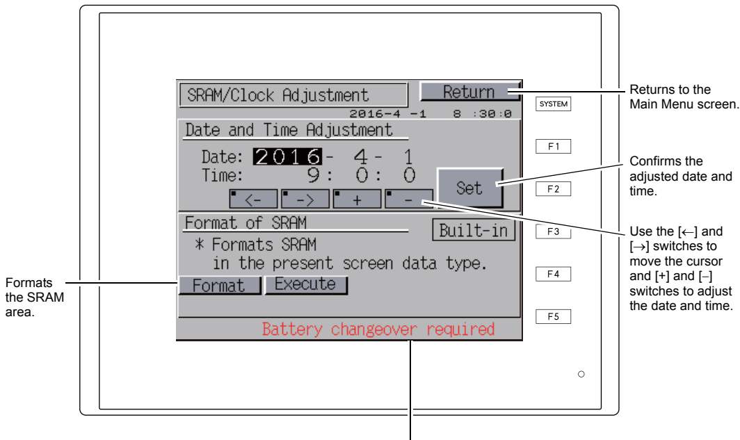
SRAM/Clock Adjustment screen
